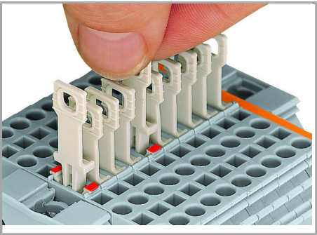
Pulling the disconnect tab by hand.
