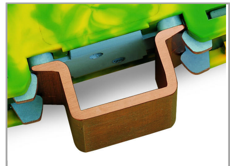
Grounding foot
