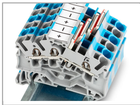
3- and 4-conductor terminal blocks (angled type)
