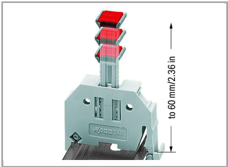
Height-adjustable group marker carrier
