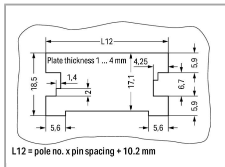
Sheet metal cutout (for female plugs without locking levers)
