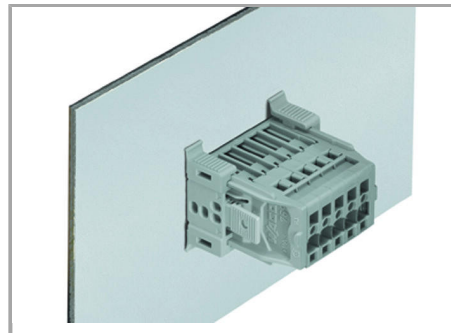
Male connector with snap-in flanges (769-605/006-000) into the cutout
