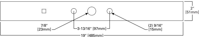
YOKE MOUNT DRILL PATTERN
