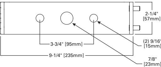
TRUNNION MOUNT DRILL PATTERN
