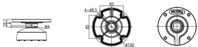
L3CPM1 Lineart
