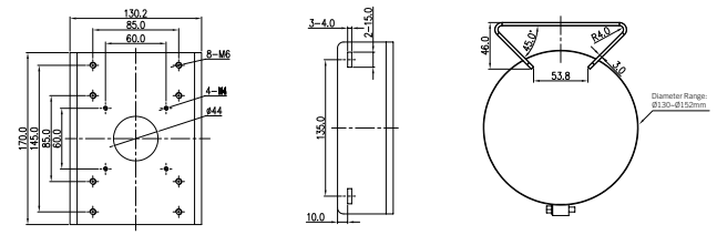
L3POLEMT2 Lineart
